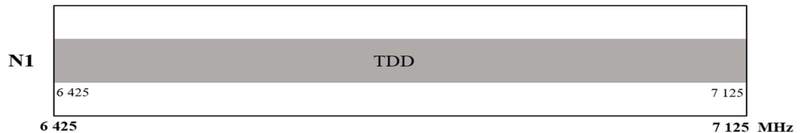
Figure 7: Frequency arrangements for N1
