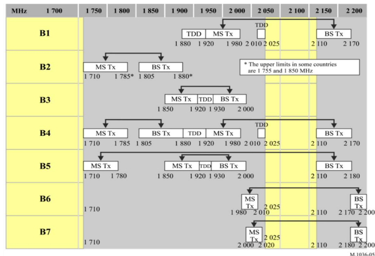
Figure 1: Frequency arrangements between 1710MHz-2200MHz
