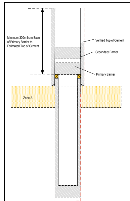
Figure D.7: Annular Cement Requirements
