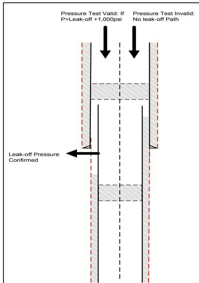
Figure D.11: Leak-off Path for Pressure Test
