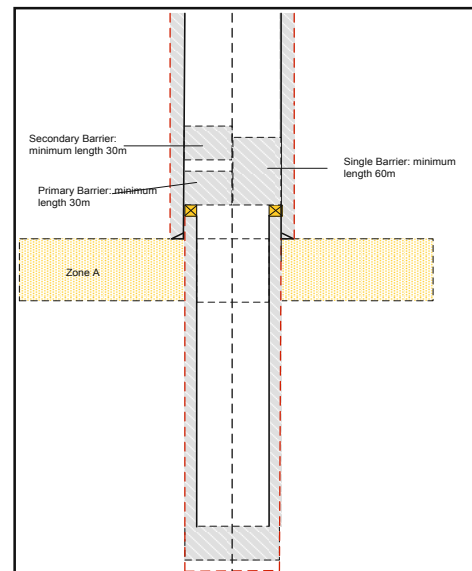
Figure D.9: Cement Plug Lengths
