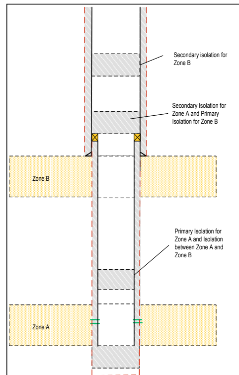
Figure D.1 Isolation of Multiple Zones
