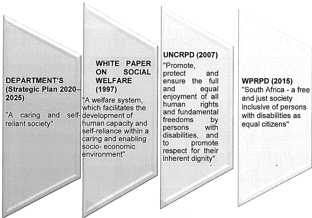
Diagram 1: Interfacing Policies
