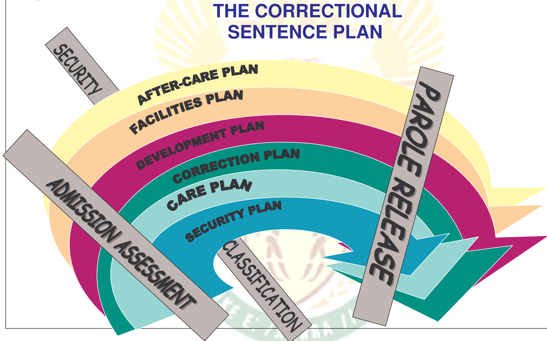
Figure 3: Sentence Plan
