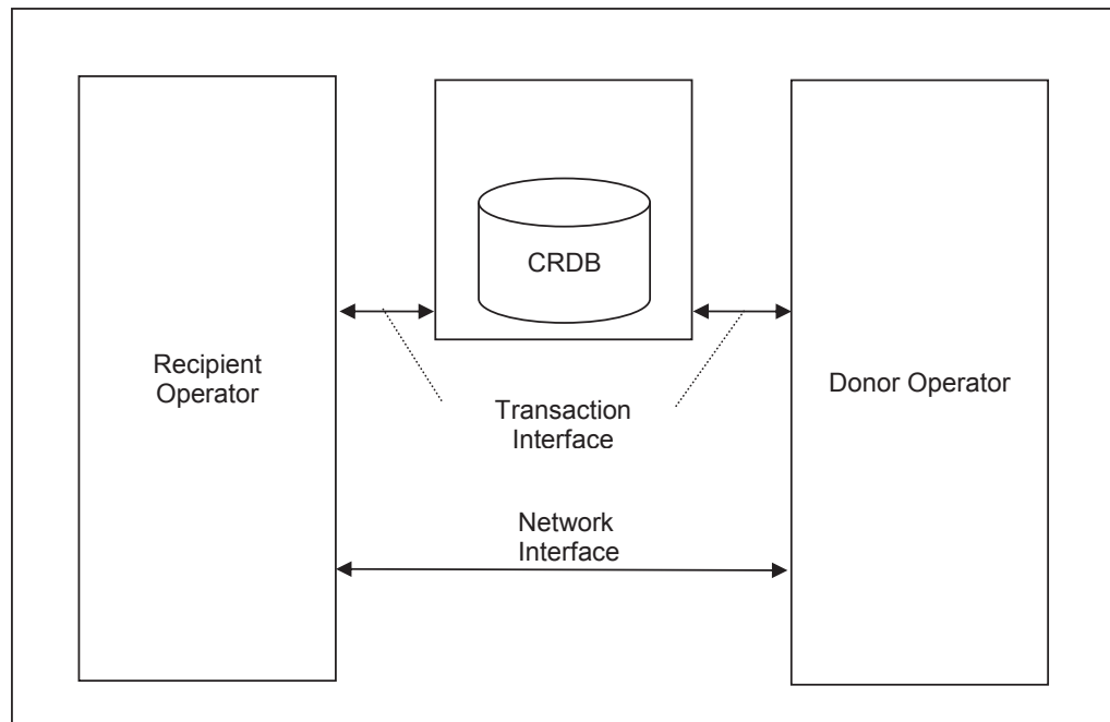
Figure 1: CRDB Architecture
