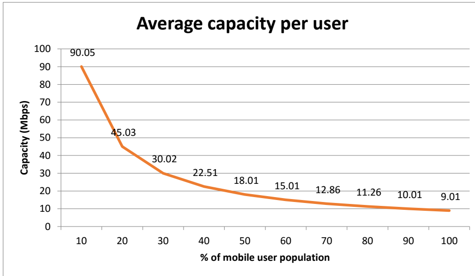
Figure 3: Average capacity per user
