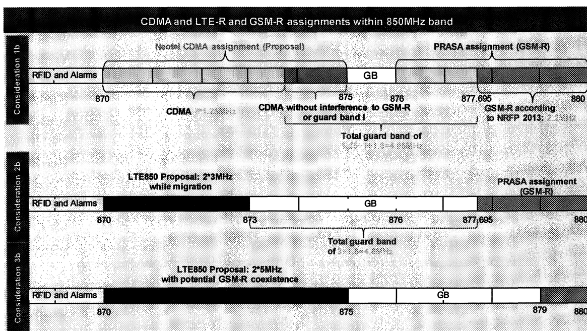
Figure 8: Migration of CDMA850 band by 2 MHz
