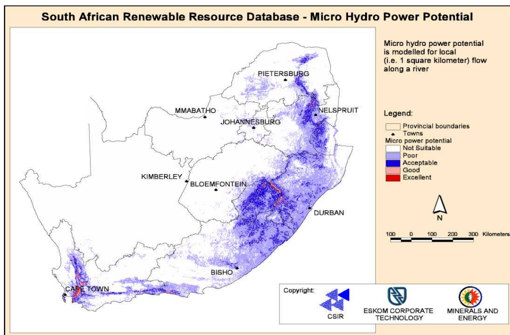
Figure 3: Areas with micro hydro potential in South Africa (DME, Eskom, CSIR, 2001)
