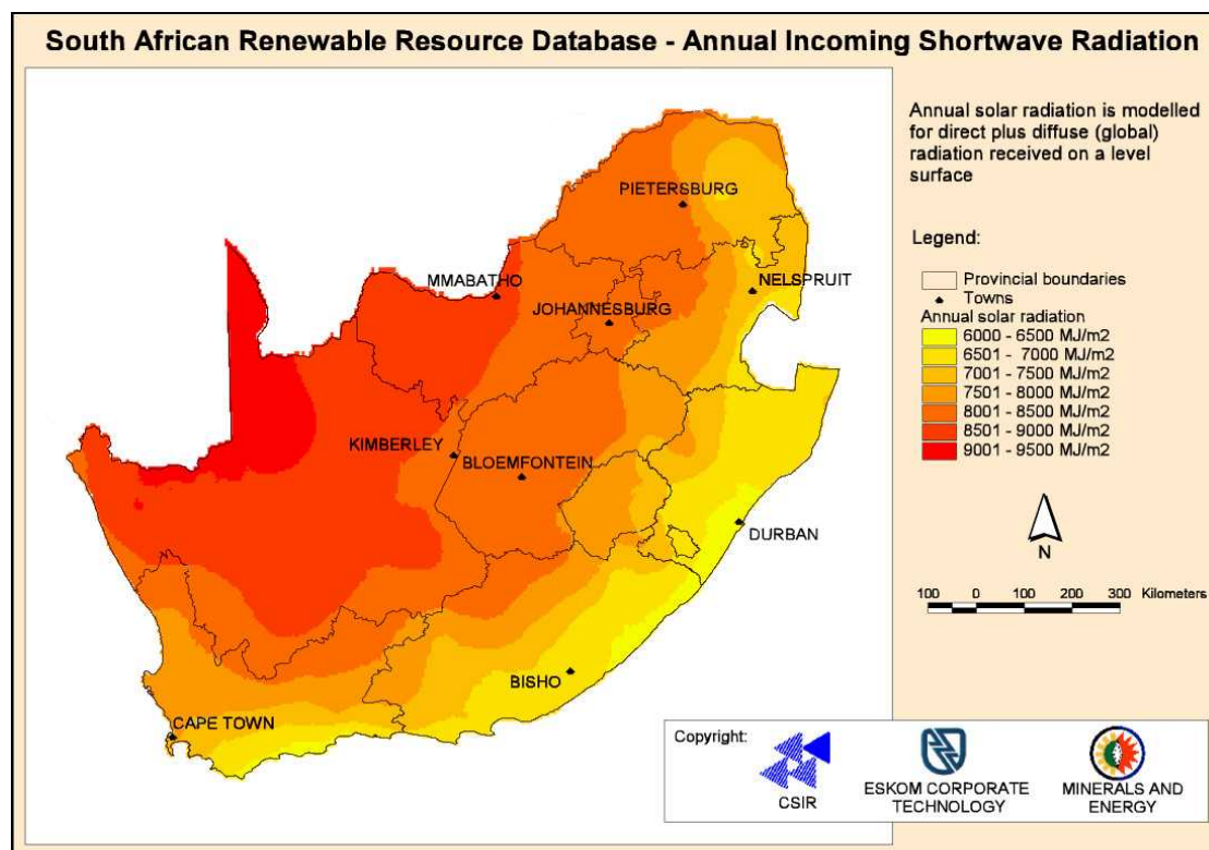
Figure 4: Annual direct and diffuse solar radiation (DME, Eskom, CSIR, 2001)
