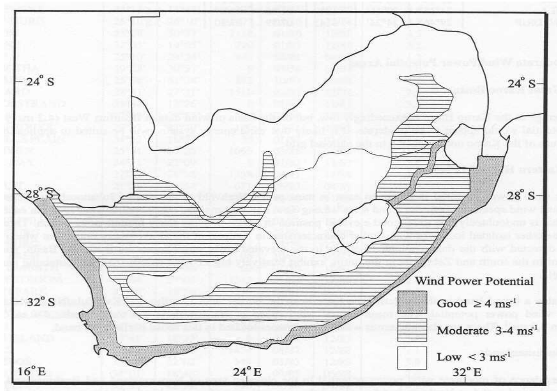
Figure 1: Generalised map of wind power potential in South Africa (Diab, 1995)
