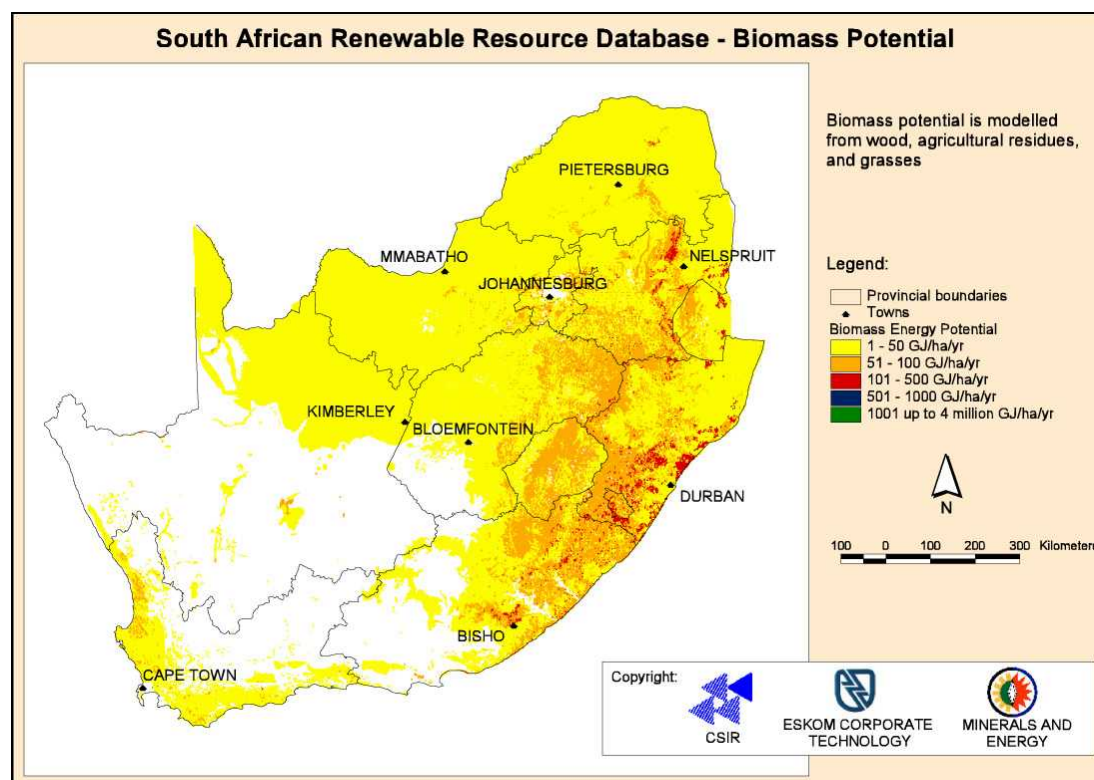
Figure 2: Total biomass energy potential for South Africa (DME, Eskom, CSIR, 2001)
