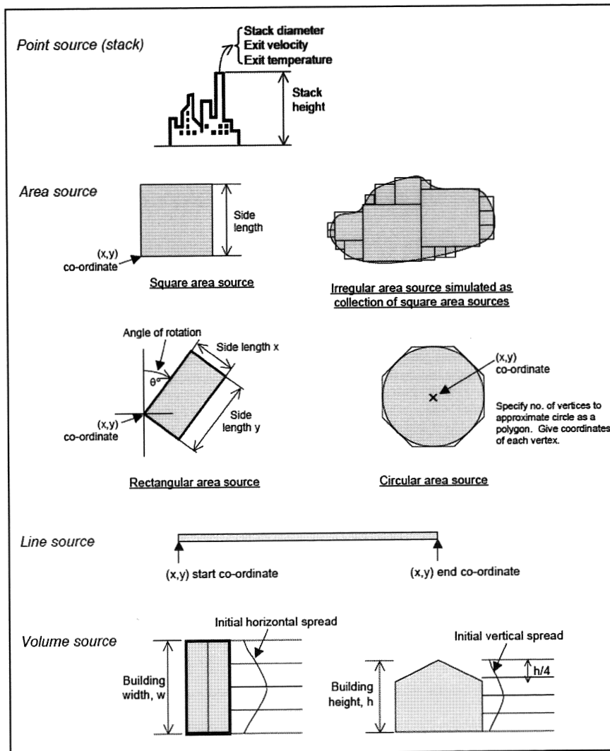
Figure 2. Types of sources used by dispersion models (New Zealand EPA 2004).
