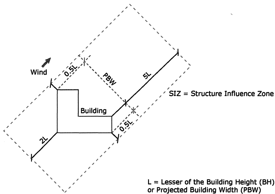
Figure 3. Structure influence zone for downwash analyses
