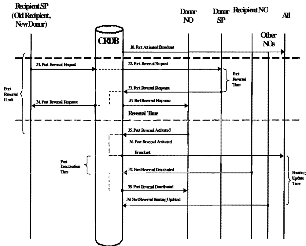
Figure 4 Schematic Illustration – Port Reversal process
