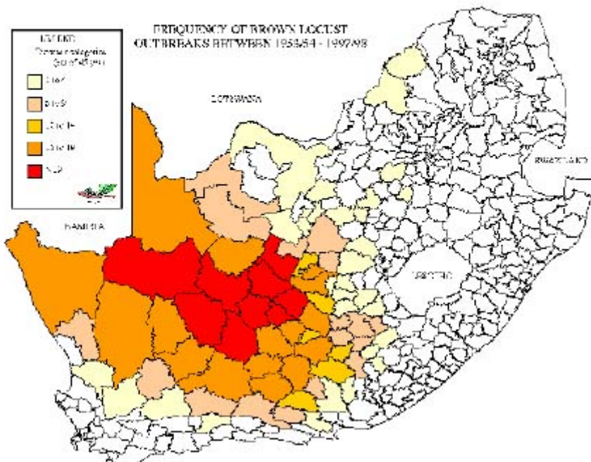
FREQUENCY OF BROWN LOCUST OUTBREAKS BETWEEN 1953/54 AND 1997/98
